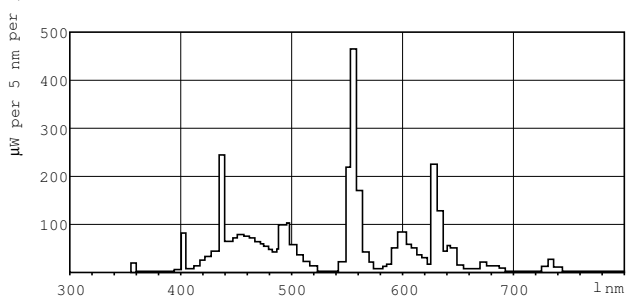
LDPB_TL5-HE8_865-Spectral power distribution B/W
